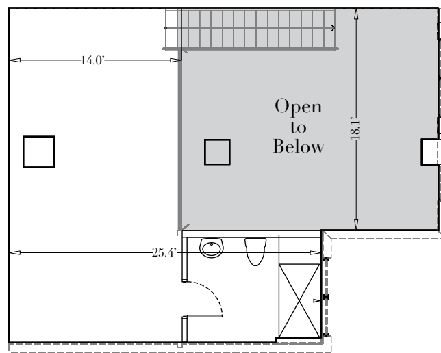
UPPER LEVEL
