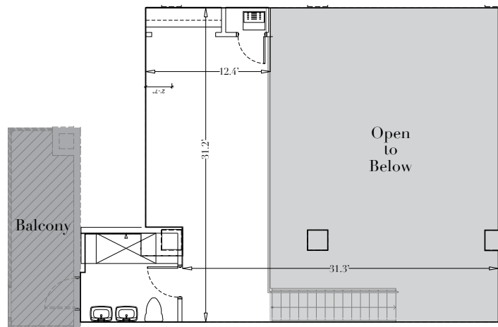
UPPER LEVEL
