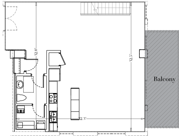
LOWER LEVEL
