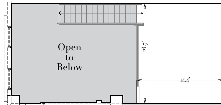
UPPER LEVEL
